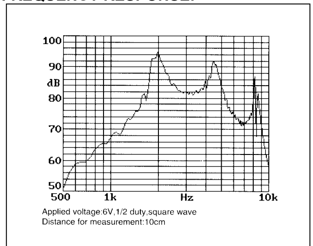
Typical curve of type MT1414-02
