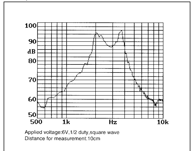
Typical curve of type MT1209-02
